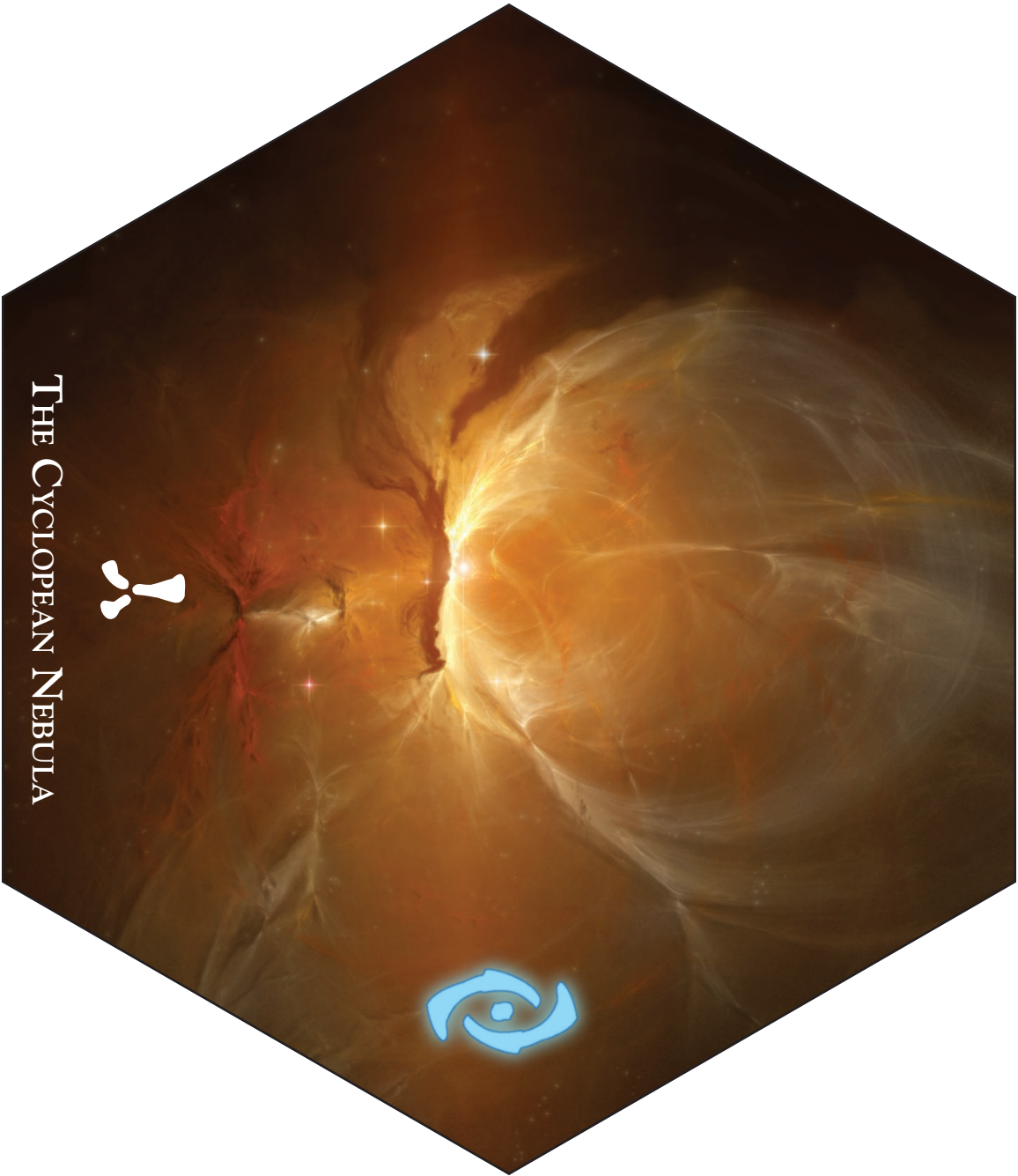
WORMHOLE
